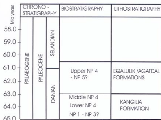
Figure 2. Stratigraphic scheme of the Early Paleocene in central Nuussuaq. The scheme is mainly based on Nøhr-Hansen et al. (2002).
