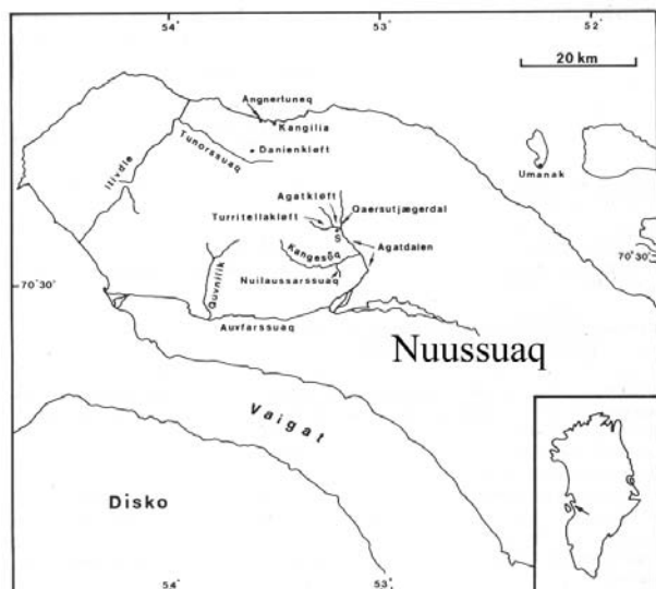
Figure 3. Localities with Paleocene molluscs on the Nuussuaq peninsula. Slightly modified from Kollmann & Peel (1983, p.7, fig. 1).
