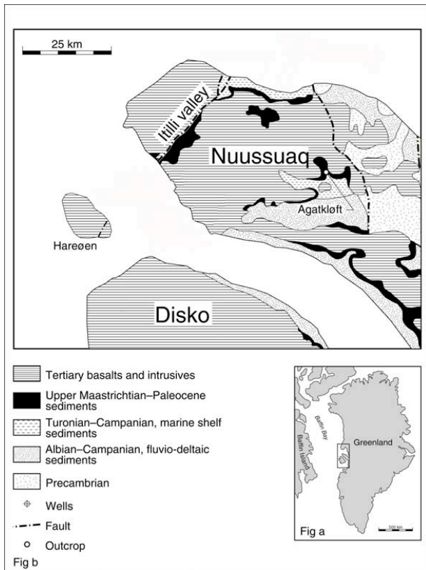
Figure 1a. Map of Greenland, showing the Nuussuaq area in the western part. Figure 1b. Geological map of the Nuussuaq Basin with the Agatkløft locality marked. Modified after Sheldon (2003) and based on GEUS maps.
