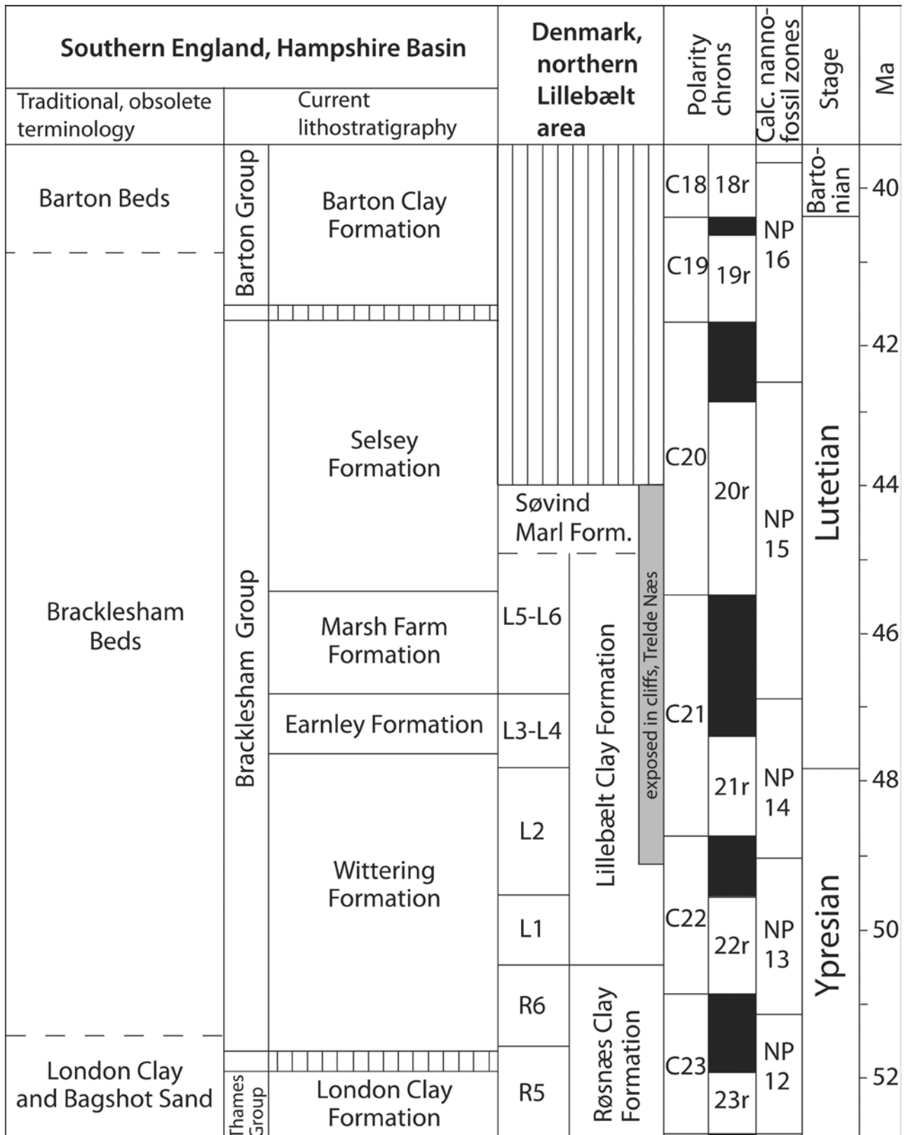
Figure 5. Correlation of the Eocene strata in the northern Lillebælt area with the succession in southern England. For convenience the older English terminology is also shown. Based in part on King (2006) and Payros et al. (2009). Only polarity chrons and calcareous nannofossil zones shown in Fig. 2 are identified in Denmark.
