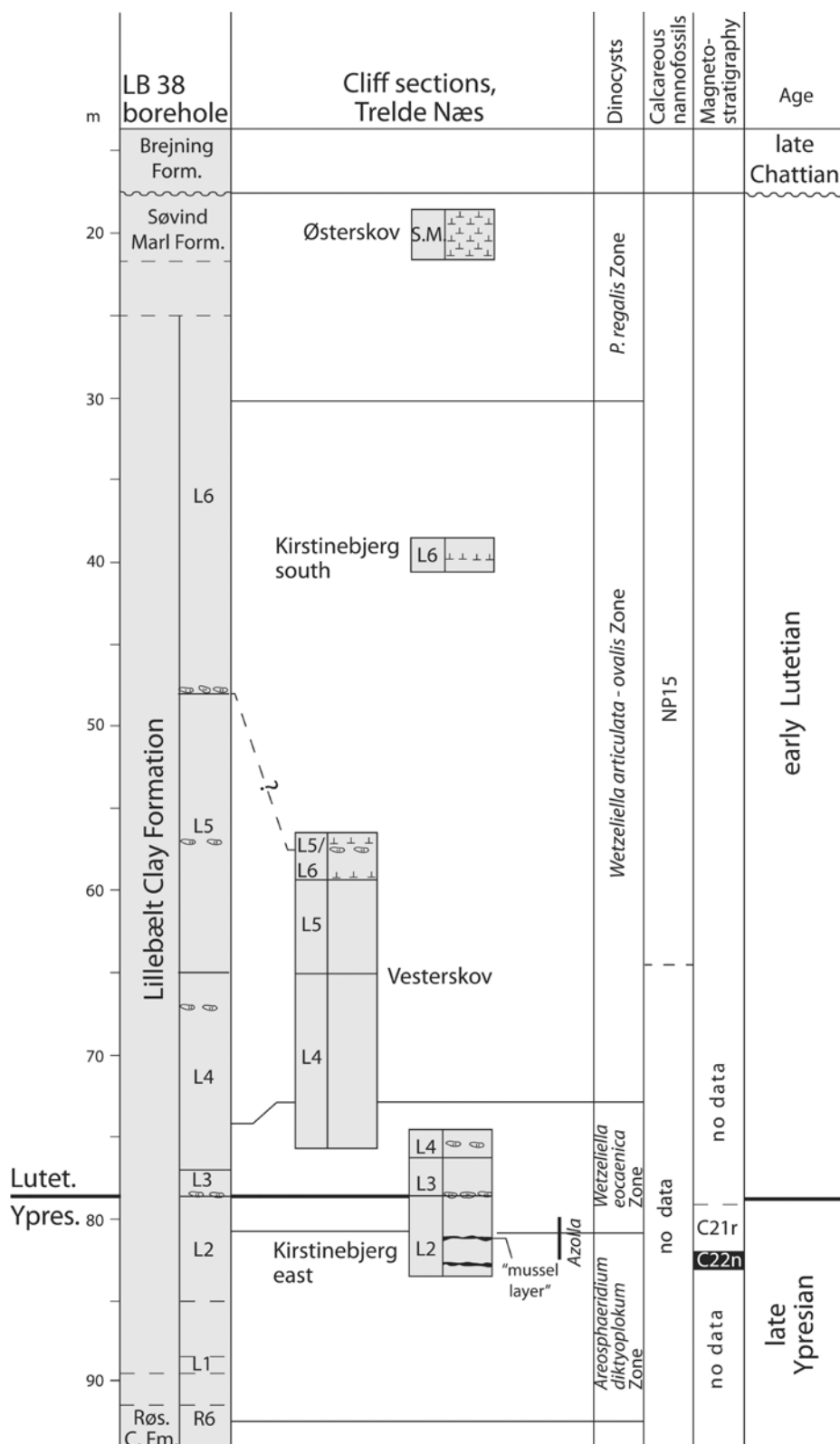
Figure 2. Logged Eocene sections on Trelde Næs and in the LB 38 borehole. All sections drawn to scale. Lithostratigraphy of LB 38 after Dinesen (1965) and Heilmann-Clausen et al. (1985). Kirstinebjerg East and Vesterskov after Heilmann-Clausen (1978). Kirstinebjerg South after Heilmann-Clausen et al. (1985); this section was not studied for dinocysts. Calcareous nannofossil data after E. Thomsen, Aarhus University (pers. comm. 2011). The dinocyst zones are defined in Heilmann-Clausen (1988). P. regalis Zone (new name for the P. geminatum Zone) (Heilmann-Clausen & van Simaey, 2005). Magnetostratigraphy after Heilmann-Clausen & Beyer (in prep.).
