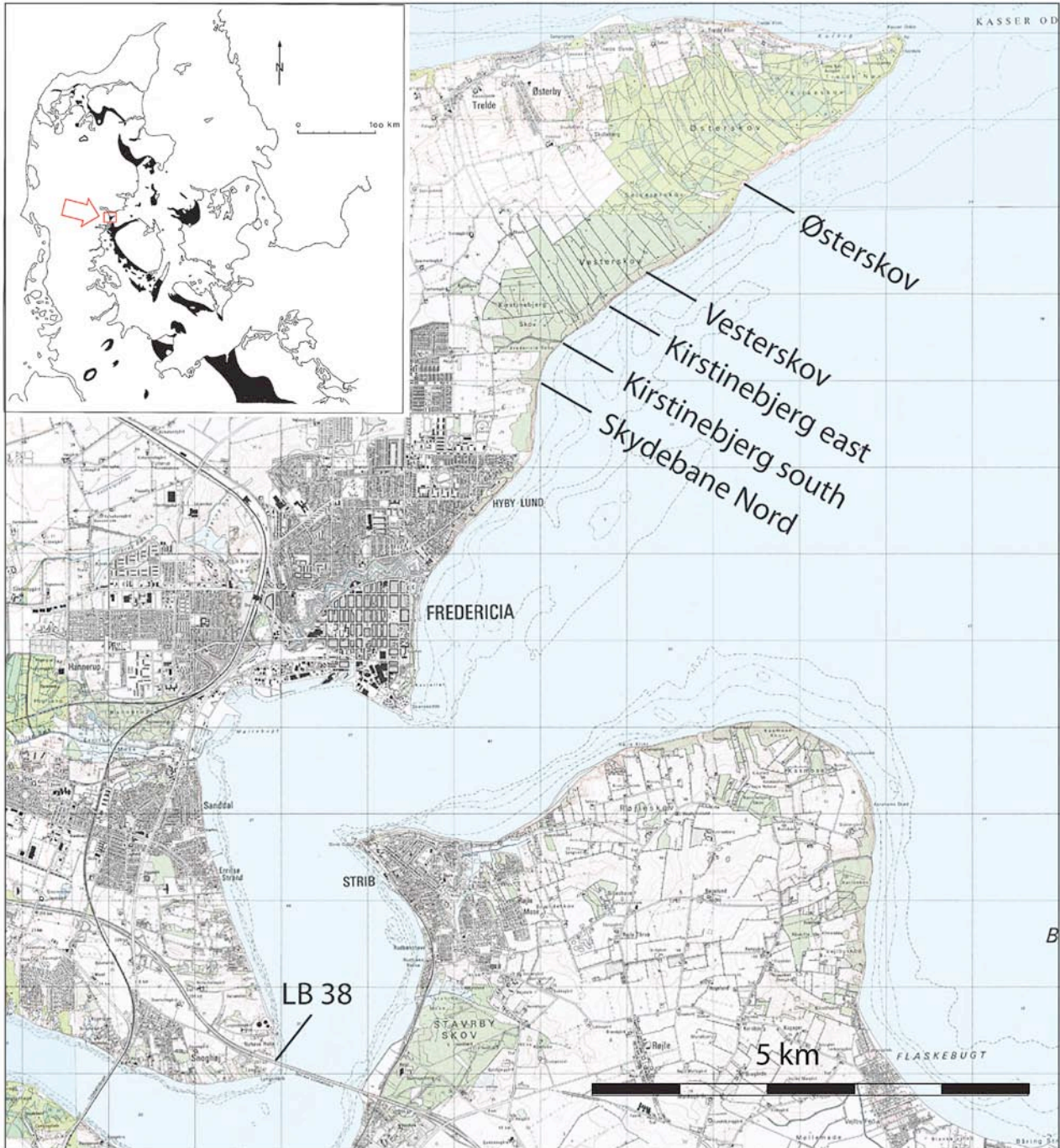
Figure 1. The Trelde Næs peninsula with localities mentioned in the text and in Fig. 2. The position of the LB 38 borehole (GEUS file no. 134.518) is also shown. The inserted map of Denmark and northern Germany shows the position of Trelde Næs (arrow). In black: Eocene subcrop (below Quaternary).
