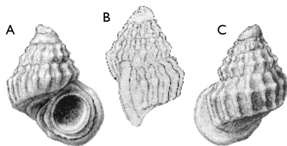
Fig. 51. Mareleptopoma ? sp. MGUH 31000 (ex Rkz 162), height 1.3 mm, width 1.0 mm.
