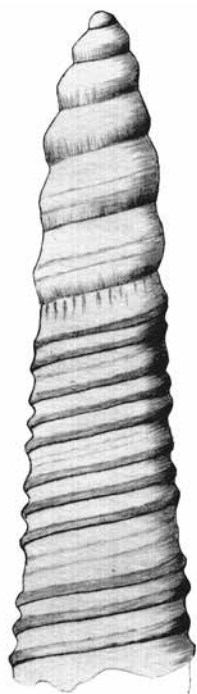
Fig. 134. Thereitis tricingulata (Ravn 1933). MGUH 3173, height 5.3 mm, width 0.8 mm.
