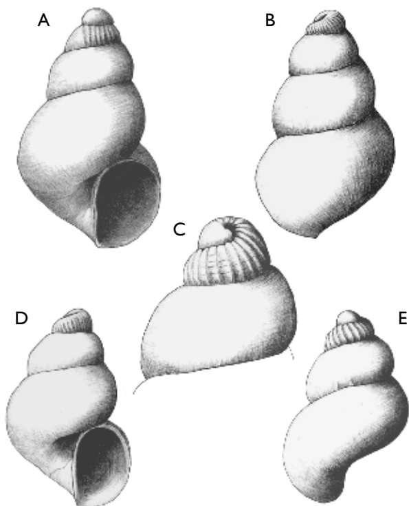
Fig. 69. Laeviphitus sp. A–C: MGUH 31023 (ex Rkz 137), height 2.2 mm, width 1.4 mm. D, E: MGUH 31024 (ex Rkz 133), height 2.2 mm, width 1.4 mm.
