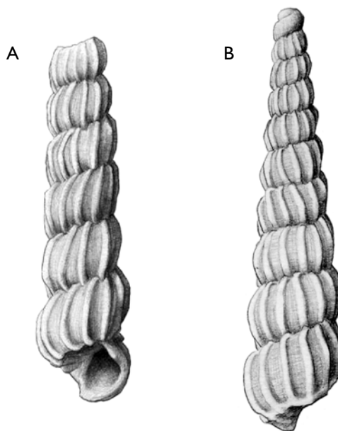
Fig. 91. Graphis sp. 1. A: MGUH 31054 (ex Rkz 50A), height 4.3 mm, width 1.1 mm. B: MGUH 31055 (ex Rkz 50B), height 4.0 mm, width 0.9 mm.
