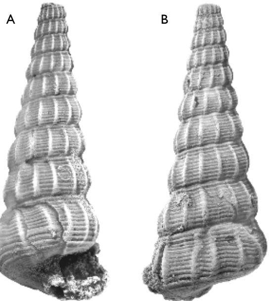
Fig. 81. Acrilla? sp. MGUH 31041 (ex ARF), height 11.5 mm, width 4.4 mm.
