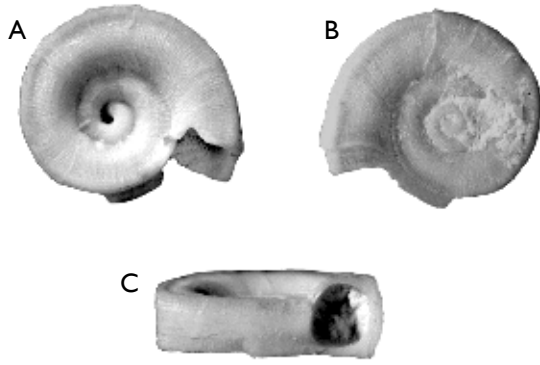
Fig. 175. Pseudomalaxis sp. MGUH 31146 (ex ARF 25127), height 1.6 mm, width 4.2 mm. Photo: Leif Rasmussen, Faxø, Denmark.
