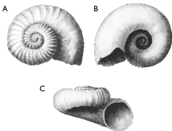
Fig. 53. Urceolabrum sp. 2. MGUH 31002 (ex Rkz 104), height 1.3 mm, width 2.2 mm.
