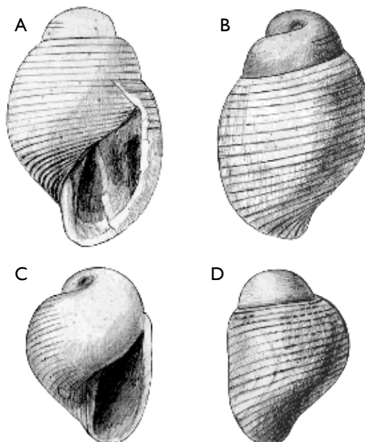
Fig. 169. Acteon sp. A, B: MGUH 31139 (ex Rkz 253), height 1.9 mm, width 1.3 mm. C, D: MGUH 31140 (ex Rkz 254), height 1.4 mm, width 1.0 mm.
