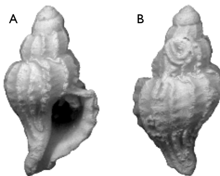
Fig. 151. Pterynotus ( Pterochelus ) sp. MGUH 31131 (ex ARF 25078), height 4.5 mm, width 1.9 mm.
