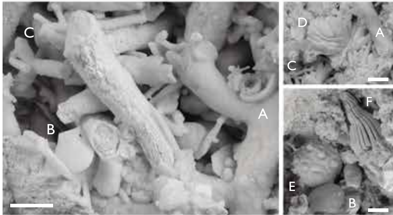
Fig. v. The rich associated fauna of the Faxe Formation is dominated by originally calcitic, shelly invertebrates. A: Moulds of the frame-building coral Dendrophyllia candelabrum . B: Two specimens of the bivalve Chlamys hennigi are well hidden between the coral branches. C: Bryozoans are also common. D: Mould of the decapod Dromiopsis rugosa which is common throughout the cold-water coral limestone. E: Echinoid plates from a Cidarid sp. Small specimens are common, being specially adapted to live in between the coral branches. F: Mould of a solitary coral. Scale bar is 10 mm.
