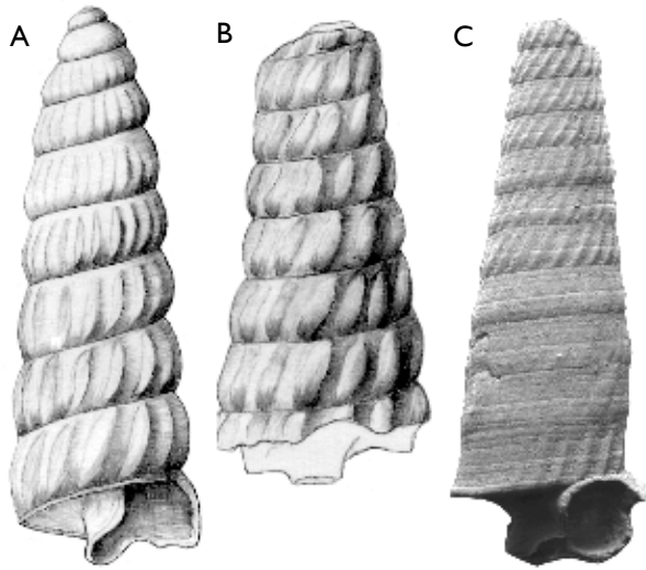
Fig. 138. Trituba obliquecostulata (Ravn 1933). A: MGUH 3159, height 2.0 mm, width 0.7 mm. B: MGUH 3160, height 2.7 mm, width 1.3 mm. C: MGUH 31073 (ex ARF 25044), height 5.2 mm, width 1.8 mm.
