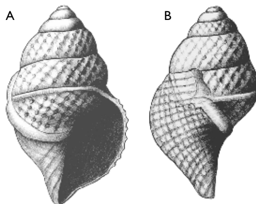
Fig. 45. Palaeocypraea sp. MGUH 30995 (ex Rkz 166), height 2.0 mm, width 1.3 mm.
