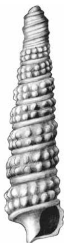
Fig. 115. Cerithiopsis sp. 10. MGUH 31090 (ex Rkz 214), height 2.9 mm, width 0.7 mm.
