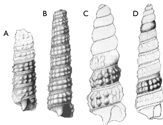
Fig. 117. Zaclys? nuetzeli n. sp. A: MGUH 31091 (ex Rkz 205), height 3.1 mm, width 0.9 mm. B: MGUH 31092 (ex Rkz 202), height 3.9 mm, width 1.0 mm. C: MGUH 3172, height 2.5 mm, width 0.8 mm. D: MGUH 31093 (ex Rkz 209), height 3.3 mm, width 0.9 mm.
