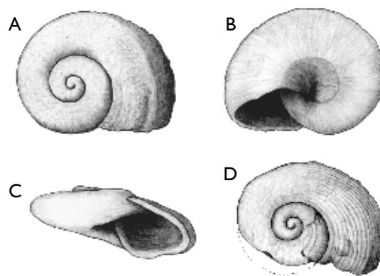
Fig. 64. Sigaretorinus sp. A–C: MGUH 31017 (ex Rkz 116), height 0.6 mm, width 1.7 mm. D: MGUH 31018 (ex Rkz 115), diameter 2.0 mm.
