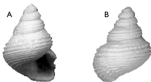
Fig. 42. Trichotropis? sp. MGUH 30993 (ex ARF 25092), height 3.7 mm, width 2.4 mm.
