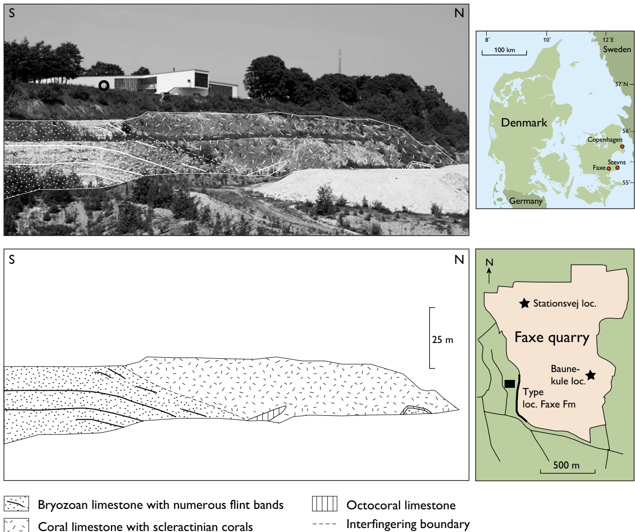
Fig. iv. Photograph and accompanying sketch of coral mounds intercalating with bryozoan mounds in the Faxe quarry at the type locality of the Faxe Formation, close to Geomuseum Faxe (GMF); two persons for scale are encircled in front of the museum. The flint layers in the bryozoan limestone emphasise the original bedding of the mounds. Octocoral limestones are rare in the quarry and are commonly found to have accumulated prior to scleractinian coral growth. The coral limestone at the type locality is predominantly of the species Dendrophyllia candelabrum but minor patches of Faksephyllia faxensis are also recorded. The two localities (Stationsvej and Baunekule) where the Baunekule facies has been recorded previously are indicated on the accompanying map. Modified from Lauridsen & Bjerager (2014).
