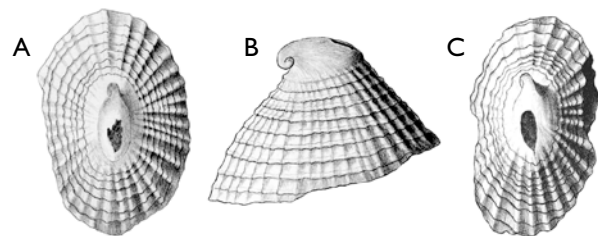
Fig. 1. Rimula? sp., A, B: MGUH 30963 (ex Rkz 154) 1.6 x 2.5 mm, 2.5 x 1.5 mm. C: MGUH 30964 (ex Rkz 154A).
