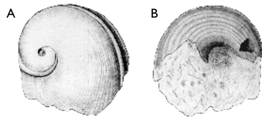
Fig. 5. Temnotropis sp. MGUH 30968 (ex Rkz 112), maximum diameter 1.9 mm.
