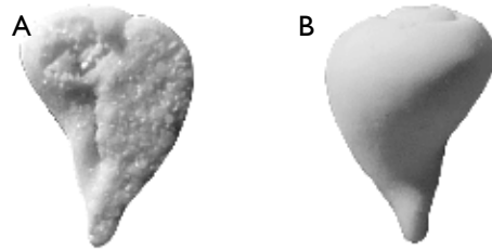
Fig. 156. Scaphella faxensis (Ravn 1902b). MGUH 31132 (ex MNO), height 7.5 mm, width 3.9 mm.
