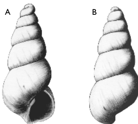
Fig. 188. Odostomia sp. 1. MGUH 31167 (ex Rkz 134), height 2.8 mm, width 1.2 mm.
