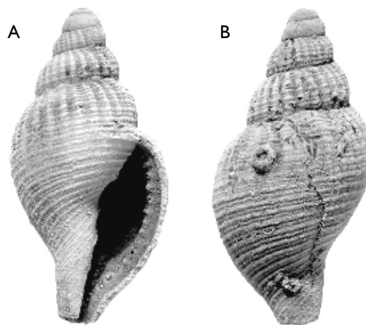
Fig. 167. Semitriton biplicatus (Ravn 1902b) MGUH 27352, height 9.8 mm, width 2.8 mm.
