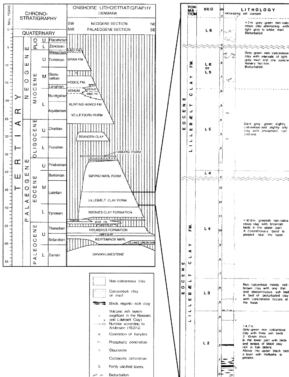
Fig. 2. Composite stratigraphic section of Lillebælt Clay Formation (right-hand column) at Trelde Næs (after Heilmann-Clausen et al., 1985, and Michelsen et al., 1998).
